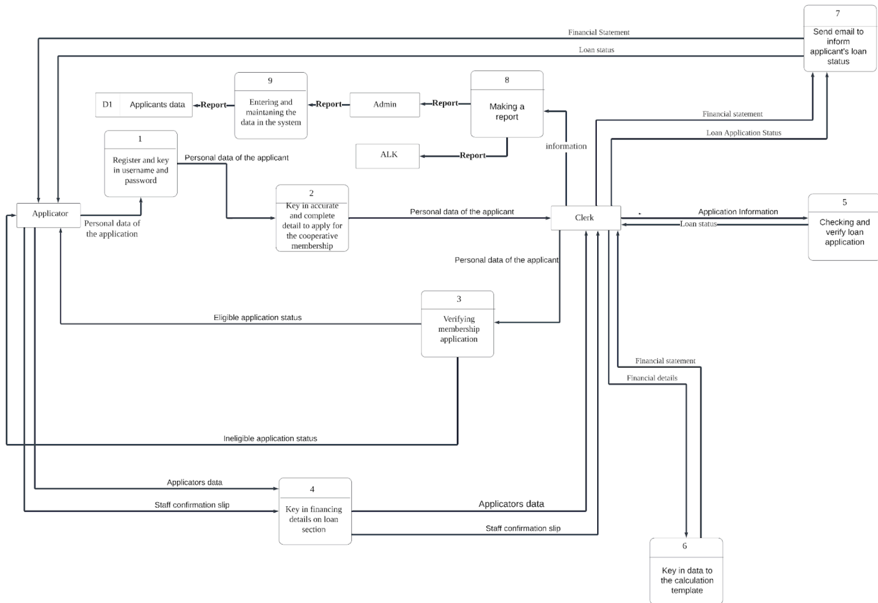
Figure 4.4.2.2 Level zero physical DFD (TO-BE) system
