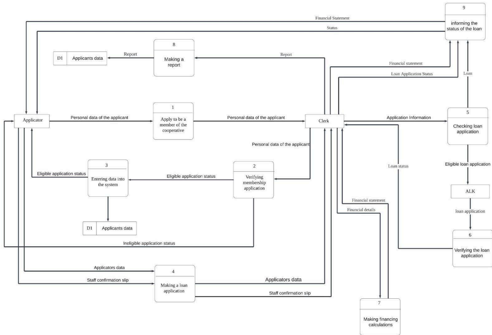
Figure 4.2.5.2 Diagram zero of the system
