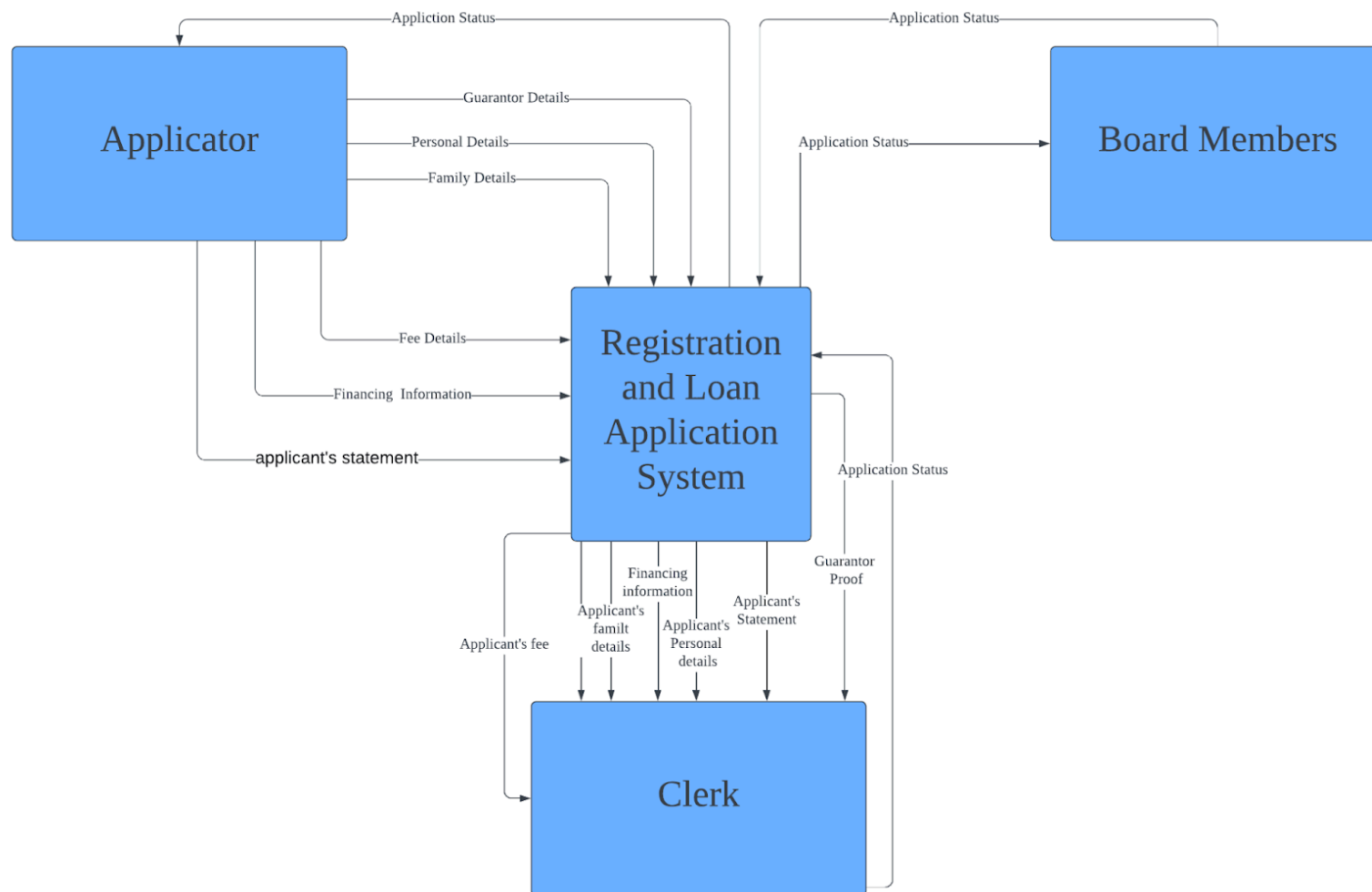
Figure 4.2.5.1 context diagram of the system
